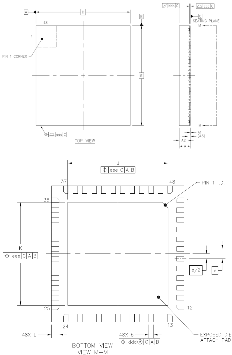
Figure 6.2. Package Drawing
